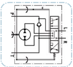
HKU.../4 4. version (OSPB...ON)
