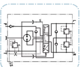
HKUS.../5T 5. version (OSPC...LS)
