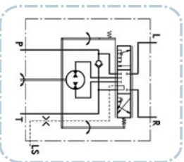
HKU.../5T 5. version (OSPB...LS)
